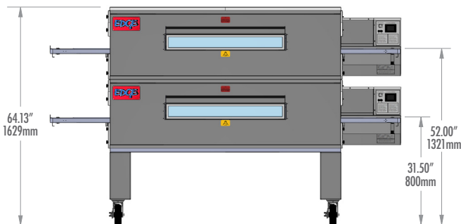
FRONT VIEW - EDGE3270-2
