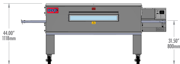
FRONT VIEW - EDGE3270-1
